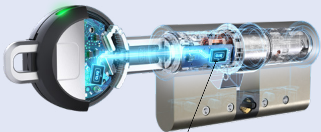
Future-proof chip generation with AES encryption and rapid processing speed with efficient energy management
